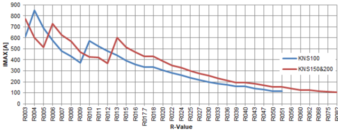
Maximum Pulse current graph KNS100 KNS150&200
