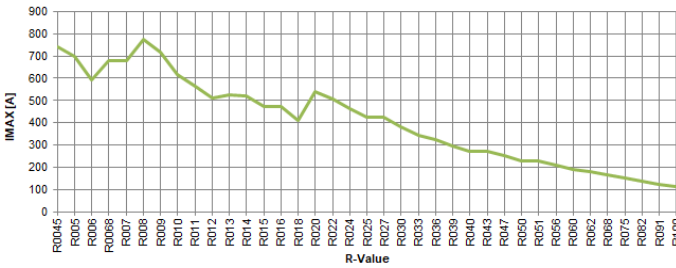
Maximum Pulse current graph KNS250
